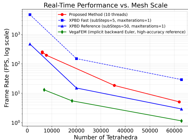
FIGURE 7. Overall-performance-trend-across-Frame rate versus mesh scalescale (log-scale FPS axis) for the proposed method (10 threads), XPBD under the Fast and Reference substep configurations defined in Section IV-A, and VegaFEM. The proposed method maintains better real-time performance than VegaFEM over a broad tetrahedral range and still retains basic interactivity on larger-scale models.
